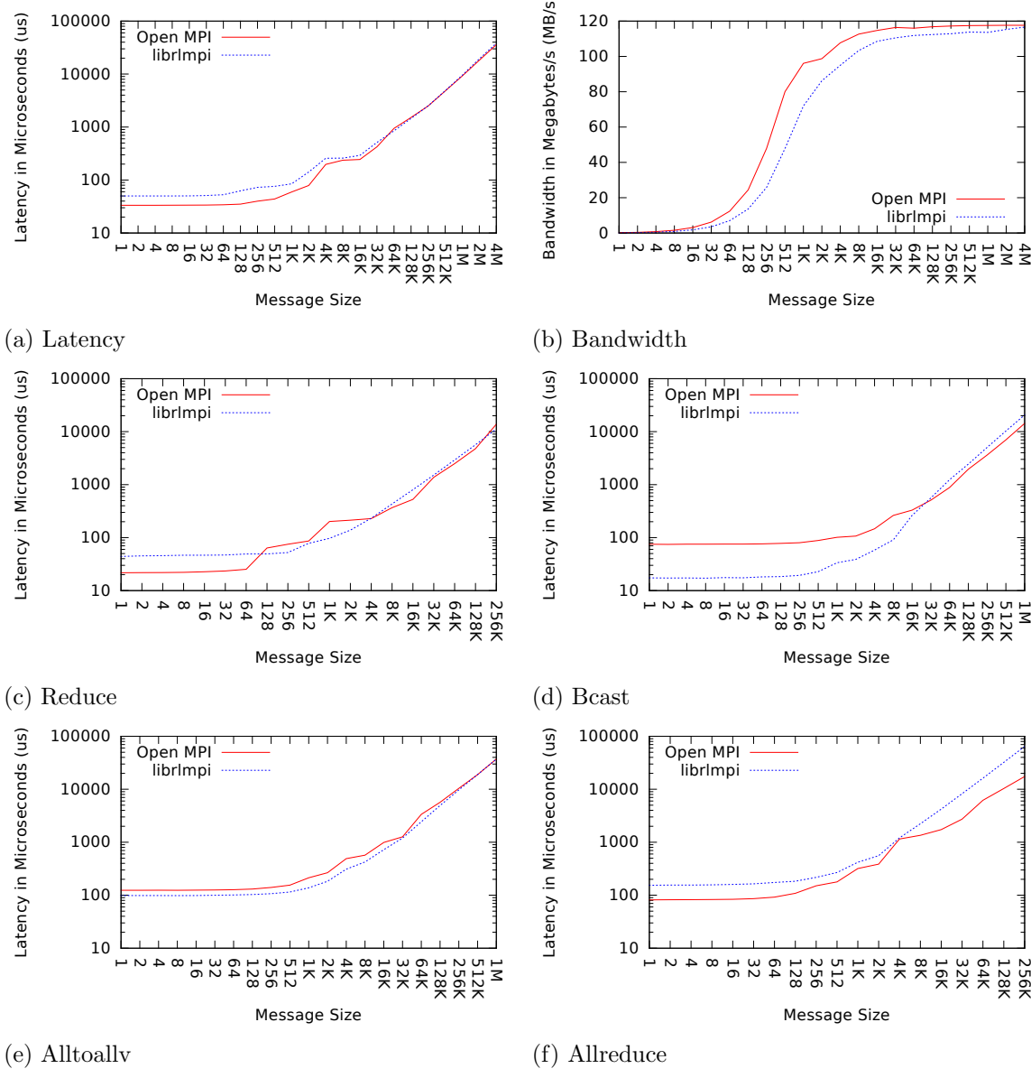
Figure 5.8 OSU Benchmarks Comparing Open MPI and liblmpi Performance
